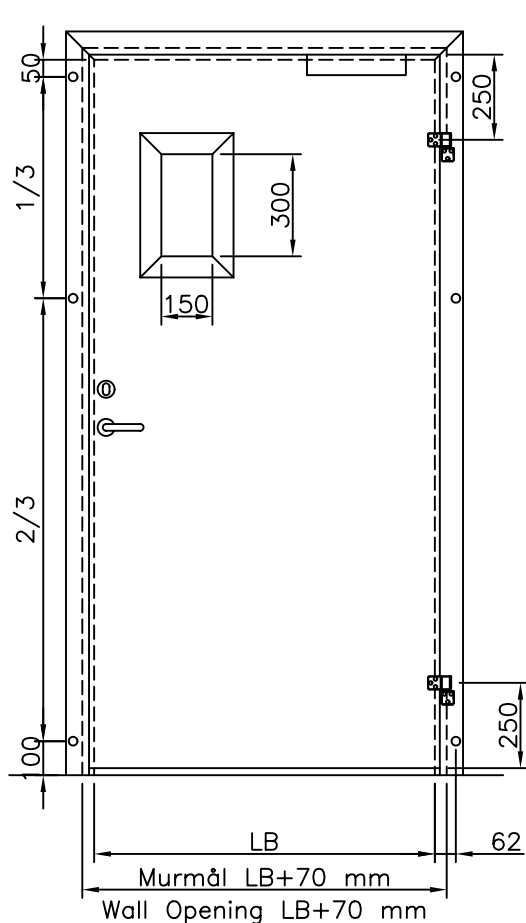
KARM TYPE C/1:5 FRAME TYPE C/1:5
