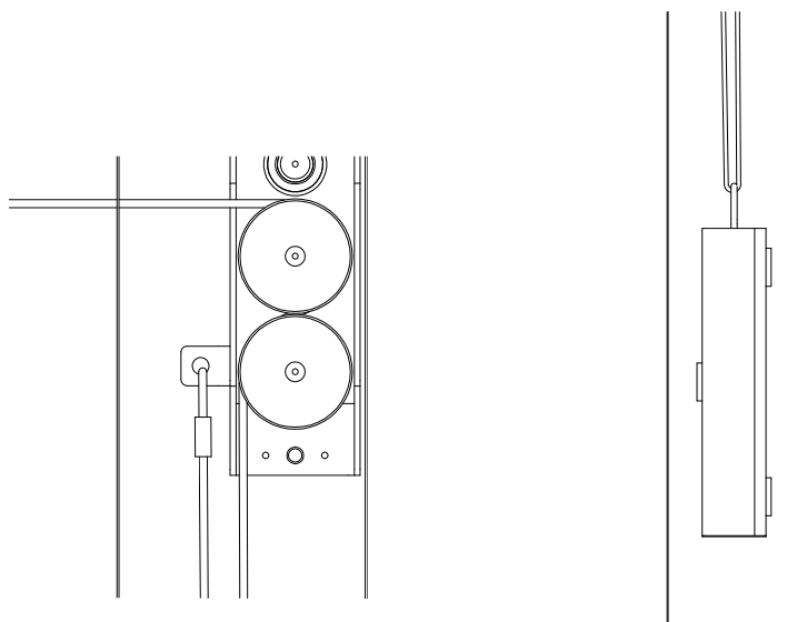
Wire by counterweight with reversing wheel
