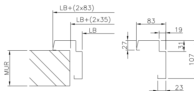
Type C2, cold store, 60/75 mm
