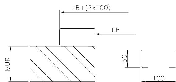
Type A1, freezer room, 100 mm
