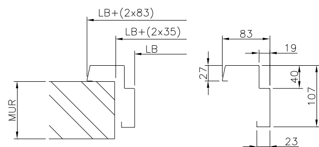
Type C, cold store, 60 mm
