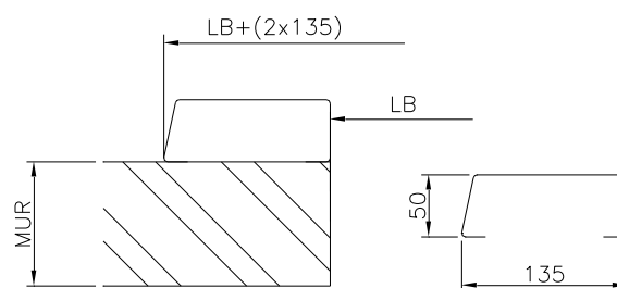
Type A, freezer room, 100/150 mm
